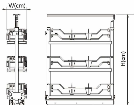
Stabilization mechanism
